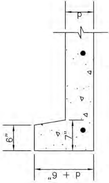
CONCRETE CURB & CONCRETE PAVEMENT
