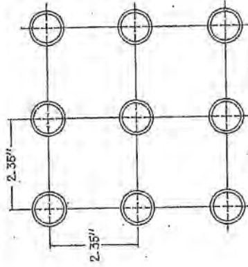
SQUARE PATTERN
