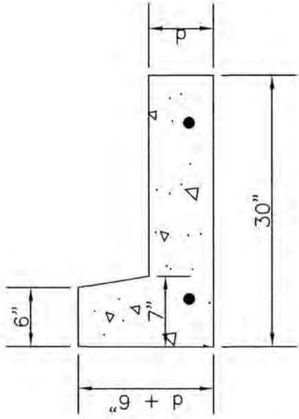
CONCRETE CURB ASPHALT PAVEMENT
